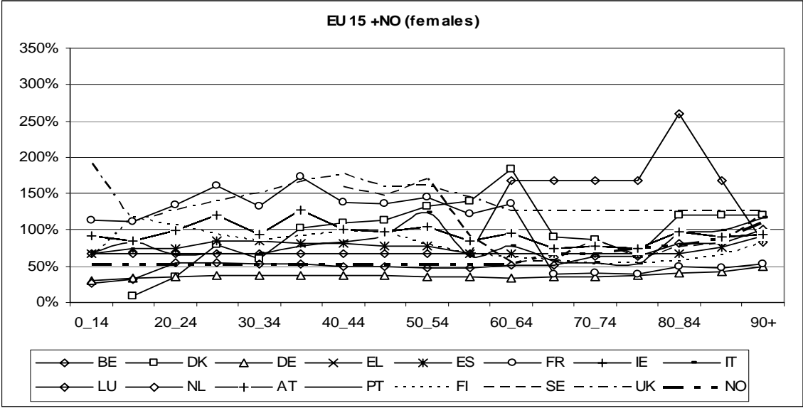
Graph 94 – Age-related expenditure profiles of long-term care provision (spending per beneficiary as % of GDP per capita)
