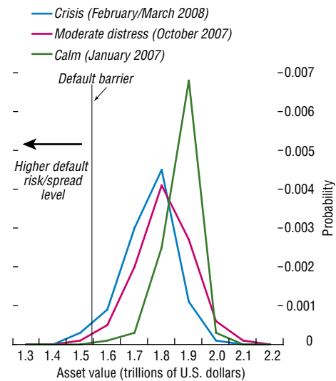
Sources: Bloomberg L.P.; Moody's KMV; and IMF staff estimates. Note: Implied asset distribution from equity option prices from Bloomberg for three dates and the default barrier estimated by Moody's KMV.
