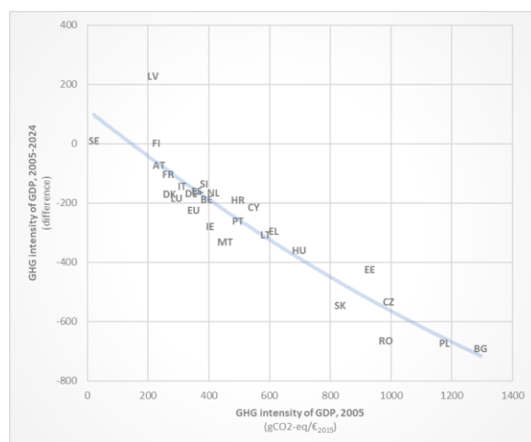
(a) GHG intensity of GDP
