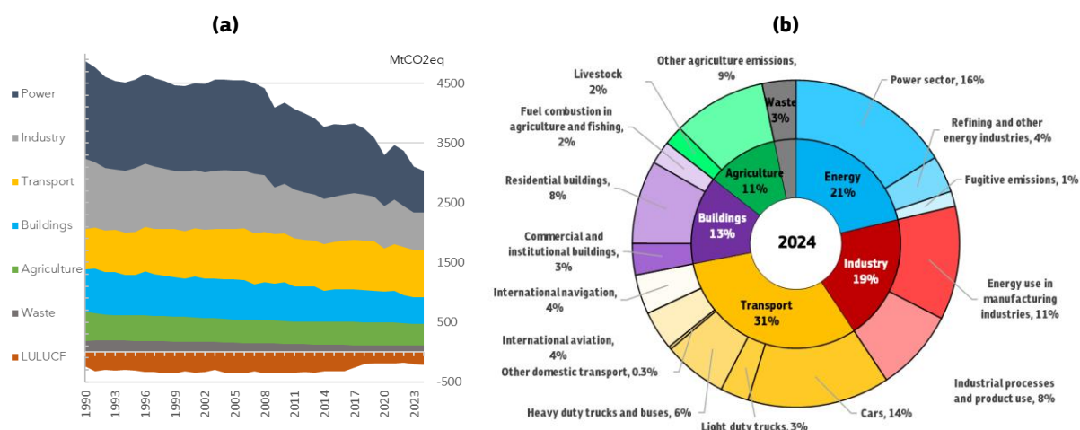
Figure 11: EU-27 greenhouse gas emissions by sector (1990-2024) and in % of total emissions (2024)
