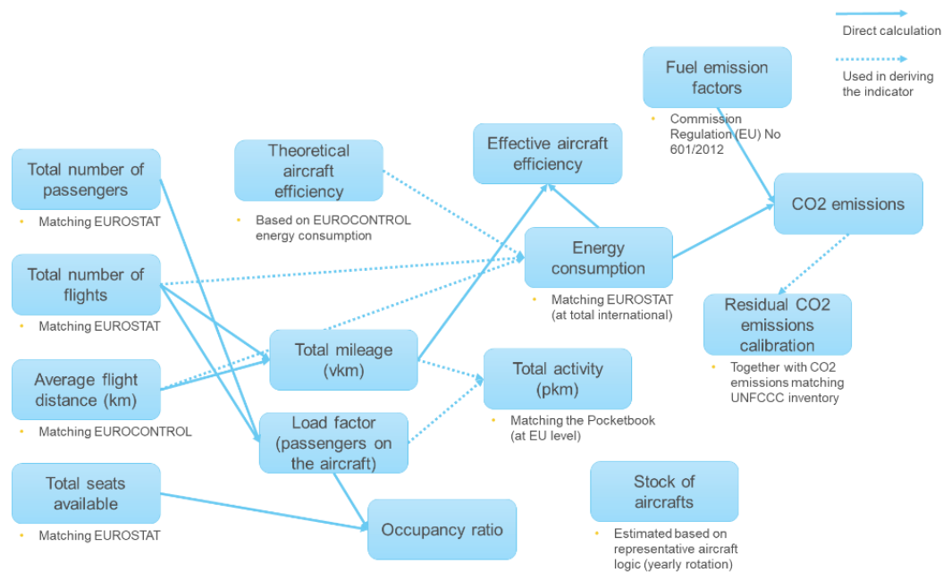
Figure 3: Aviation emissions - overview of the methodology
