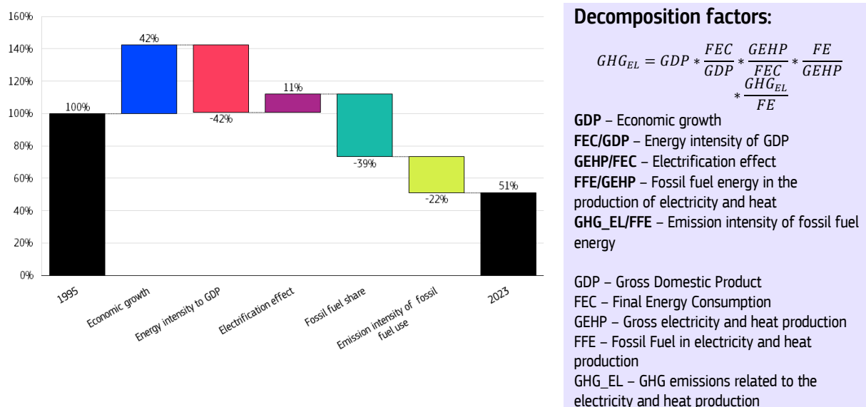
Figure 17: Decomposition of emission in electricity and heat production (1995-2023)
