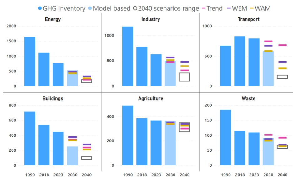
Figure 13: Past and expected emission reductions by sectors
