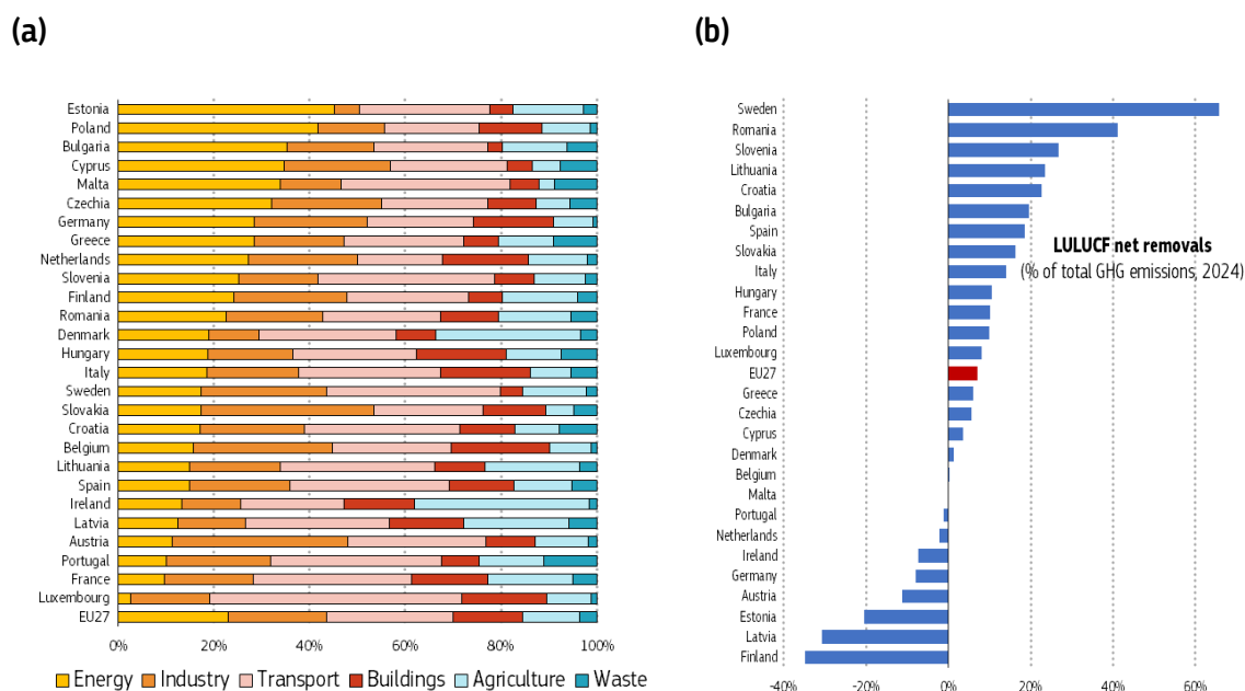
Figure 12: EU Member States greenhouse gas emissions by sector 2024 (a) and LULUCF net removals (b), in % of total emissions
