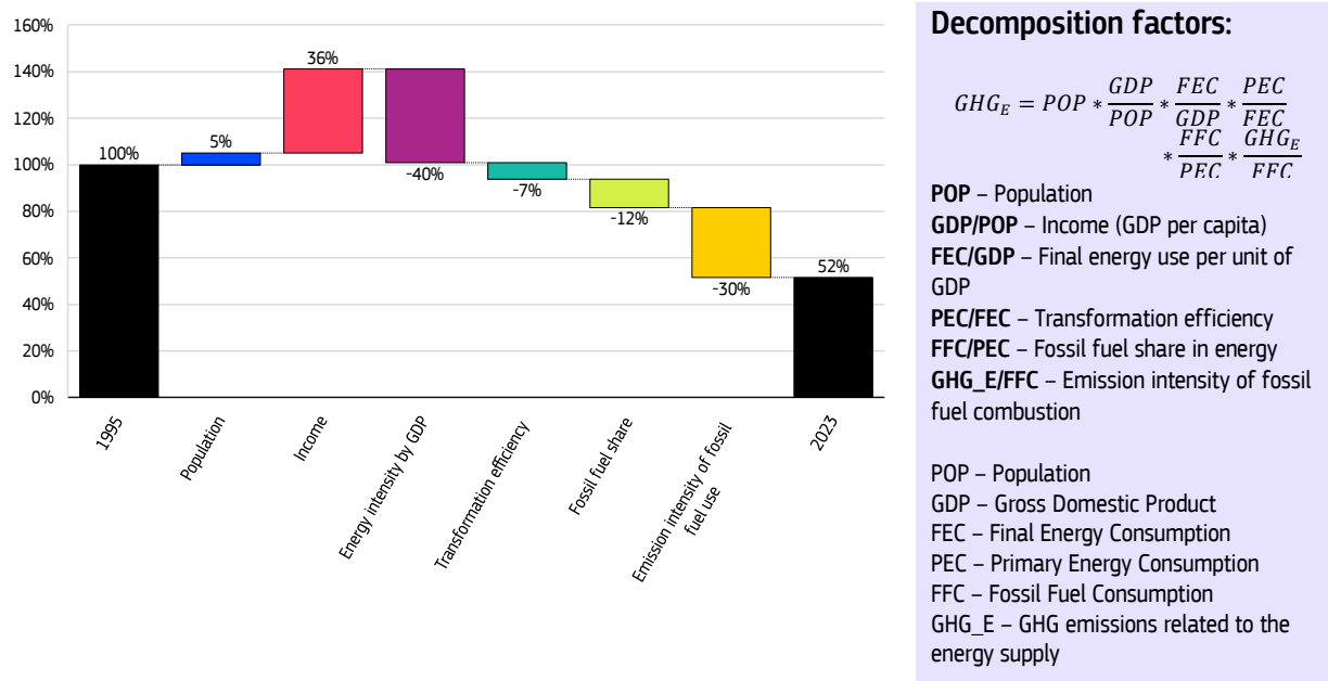
Figure 16: Decomposition of emission in energy consumption (1995-2023)
