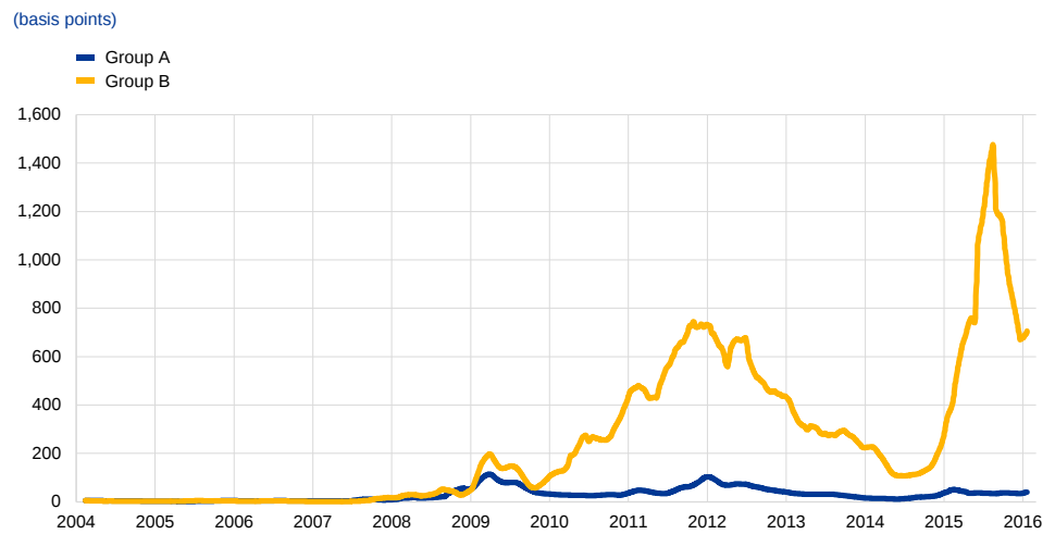
Chart S35
