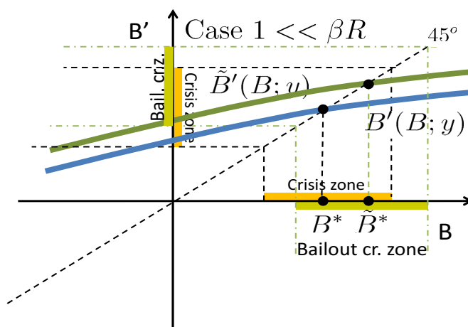
Figure 30. The stationary debt dynamics for small income fluctuations and probabilistic bailout agency
