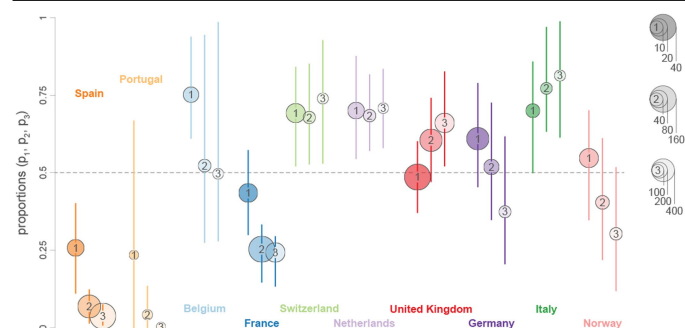
Fig. 2 | Posterior estimates for the relative importance of lineage introduction events in 10 European countries and their association with incidence. We report three summaries (posterior mean and 95% HPD intervals) for each country: the ratio of unique introductions over the total number of unique persisting lineages and unique introductions between June 15 th and August 15 th , 2020 ( p_1 ), the ratio of descendant lineages from these unique introduction events over the total number of descendants circulating on August 15 th , 2020 ( p_2 ), and the ratio of descendant taxa from these unique introductions over the total number of descendant taxa sampled after August 15 th , 2020 ( p_3 ) (cfr. Extended Data Figure 4). The dot sizes are proportional to: (1) the total number of unique lineage introductions identified between June 15 th and August 15 th , 2020, (2) the total number of lineages inferred on August 15 th , 2020, and (3) the total number of descendant tips after August 15 th , 2020.
