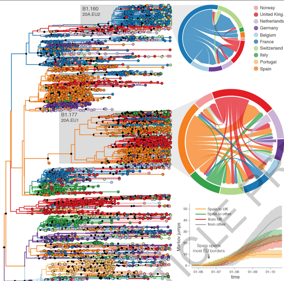
Fig. 3 | Phylogeographic estimates of SARS-CoV-2 spread in 10 European countries. The tree on the left represents the maximum clade credibility tree summary of the Bayesian inference. Colours correspond to the countries in the legend. The two clades corresponding to B1.160/20A.EU2 and B1.177/20A.EU1 are highlighted in grey. The circular migration flow plots for these variants are based on the posterior expectations of the Markov jumps. In these plots,
