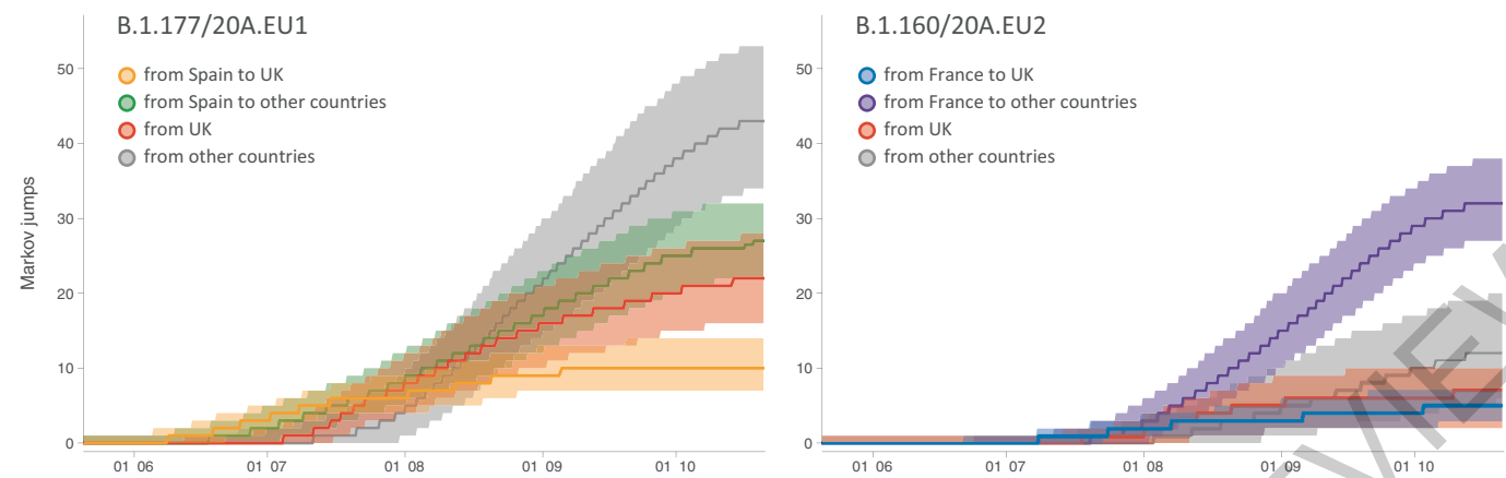
Extended Data Fig. 7 | Phylogeographic transitions for lineages B1.1777/20A.EU1 and B1.160/20A.EU2. Cumulative phylogeographic transitions are summarized as posterior mean estimates with 95% HPD intervals over time for four types of Markov jumps. For B1.1777/20A.EU1: i)
