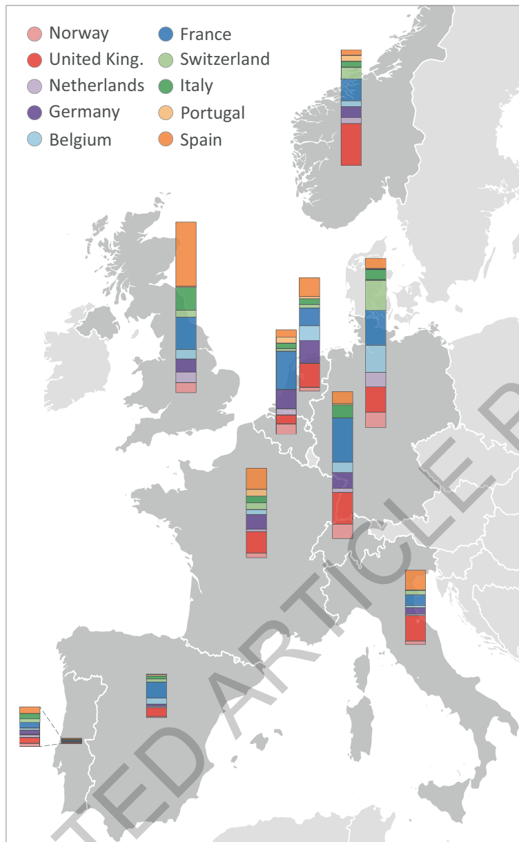
Extended Data Fig. 6 | Estimated geographic origin of viral influx over the summer (June 15 th - August 15 th , 2020) in each country. Each bar plot summarizes the posterior Markov jump estimates into a specific country. For the bar representing a low number of introductions into Portugal, a magnified view is provided.
